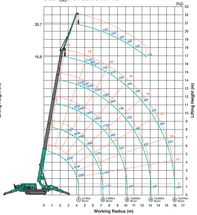
Outriggers Position : Mid
