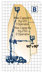
crosspieces fully extended front sector
